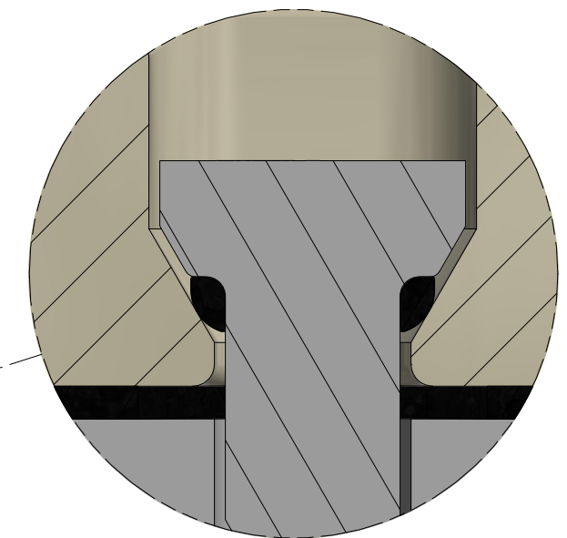
SEAL PRIOR TO DEFORMATION
