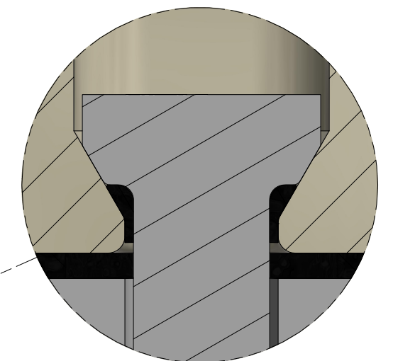
SEAL AFTER DEFORMATION
